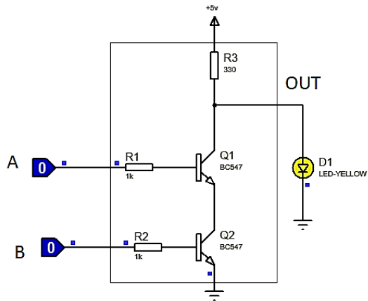
Fig.: NAND gate
