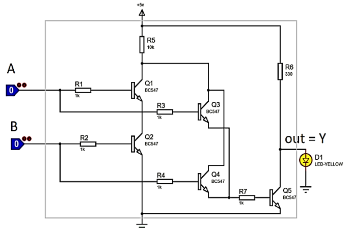
Fig.: XNOR gate
