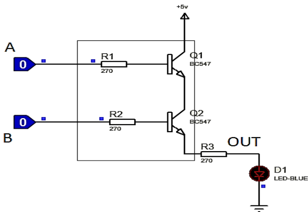
Fig.: AND gate
